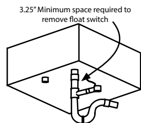
Figure 1: Vertical Drain Outlet Installation
